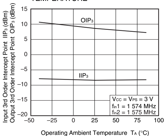
IIP 3 , OIP 3 vs. OPERATING AMBIENT TEMPERATURE
