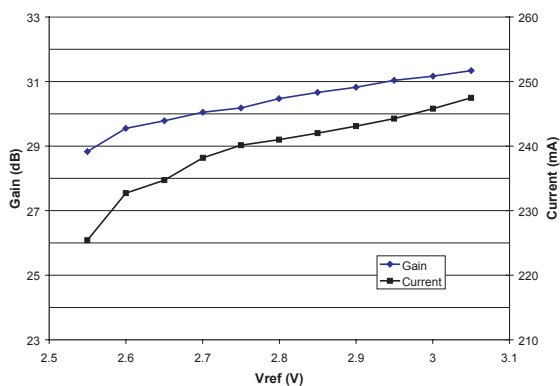
Figure 8: Gain and Current Consumption vs. V_{REF} ( T_A = +25^\circ\text{C} , V_{CC} = +5\text{ V} , f = 2472\text{ MHz} , P_{OUT} = +25\text{ dBm} , 54 Mbps 802.11g)
