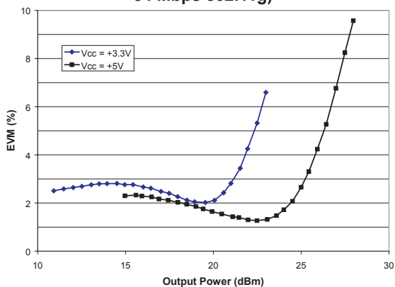
Figure 10: EVM vs. Output Power ( T_A = +25^\circ\text{C} , V_{REF} = +2.85\text{ V} , f = 2472\text{ MHz} , 54 Mbps 802.11g)
