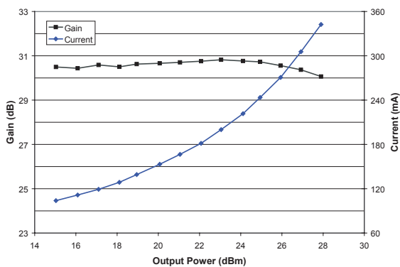
Figure 6: Gain and Current Consumption vs. Output Power ( T_A = +25\text{ }^{\circ}\text{C} , V_{CC} = +5\text{ V} , V_{REF} = +2.85\text{ V} , f = 2472\text{ MHz} , 54 Mbps 802.11g)
