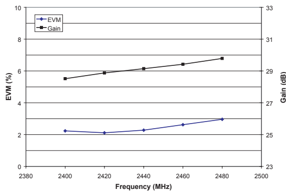
Figure 3: EVM and Gain vs Frequency ( T_A = +25\text{ }^{\circ}\text{C} , V_{CC} = +3.3\text{ V} , V_{REF} = +2.85\text{ V} , P_{OUT} = +21\text{ dBm} , 54 Mbps 802.11g)
