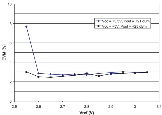
Figure 9: EVM vs V_{REF} ( T_A = +25^\circ\text{C} , f = 2472\text{ MHz} , 54 Mbps 802.11g)
