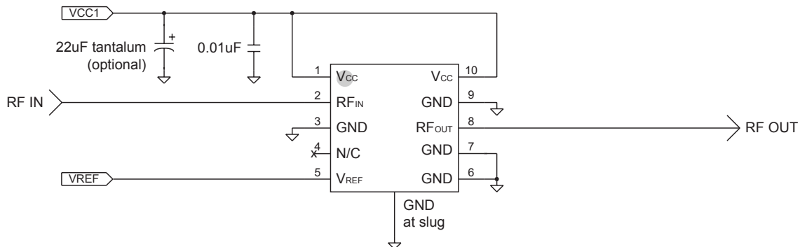
Figure 11: Application Circuit
