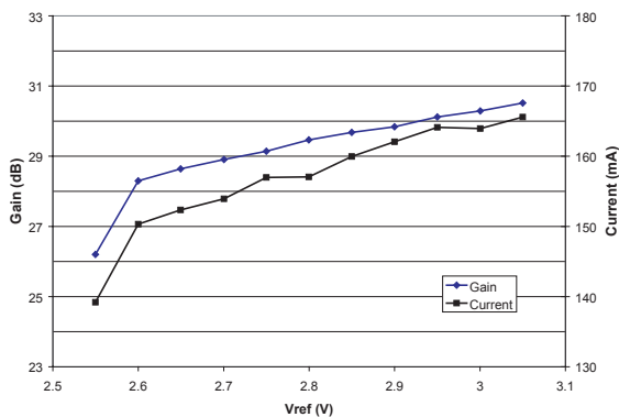
Figure 7: Gain and Current Consumption vs. V_{REF} ( T_A = +25^\circ\text{C} , V_{CC} = +3.3\text{ V} , f = 2472\text{ MHz} , P_{OUT} = +21\text{ dBm} , 54 Mbps 802.11g)
