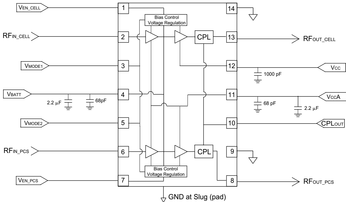
Figure 4: Application Circuit
