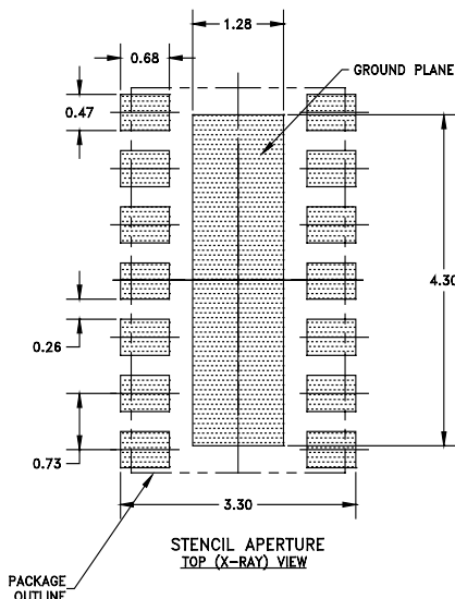
Figure 7: PCB Board Design Guidelines
