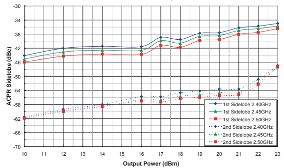
Figure 11: ACPR 1st and 2nd Sidelobe vs. Output Power Across Frequency ( V_{CC} = +3.3\text{ V} , T_c = 25^\circ\text{C} ) 802.11b Root Cosine Filtering ( \alpha = 0.50 ), 1Mbps
