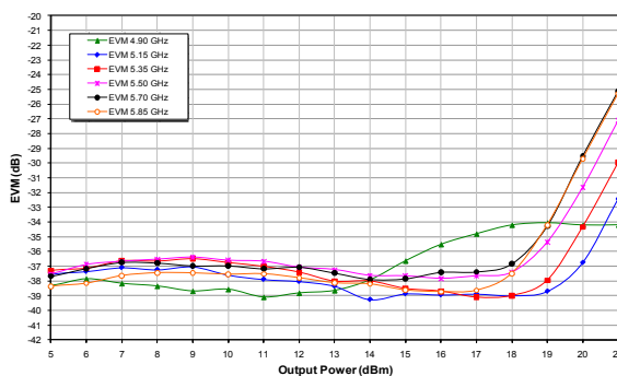
Figure 22: Tx Path Dynamic EVM vs. Output Power Across Frequency ( V_{cc} = +3.3 V, Temp = -40 °C, 802.11a, 54 Mbps OFDM)
