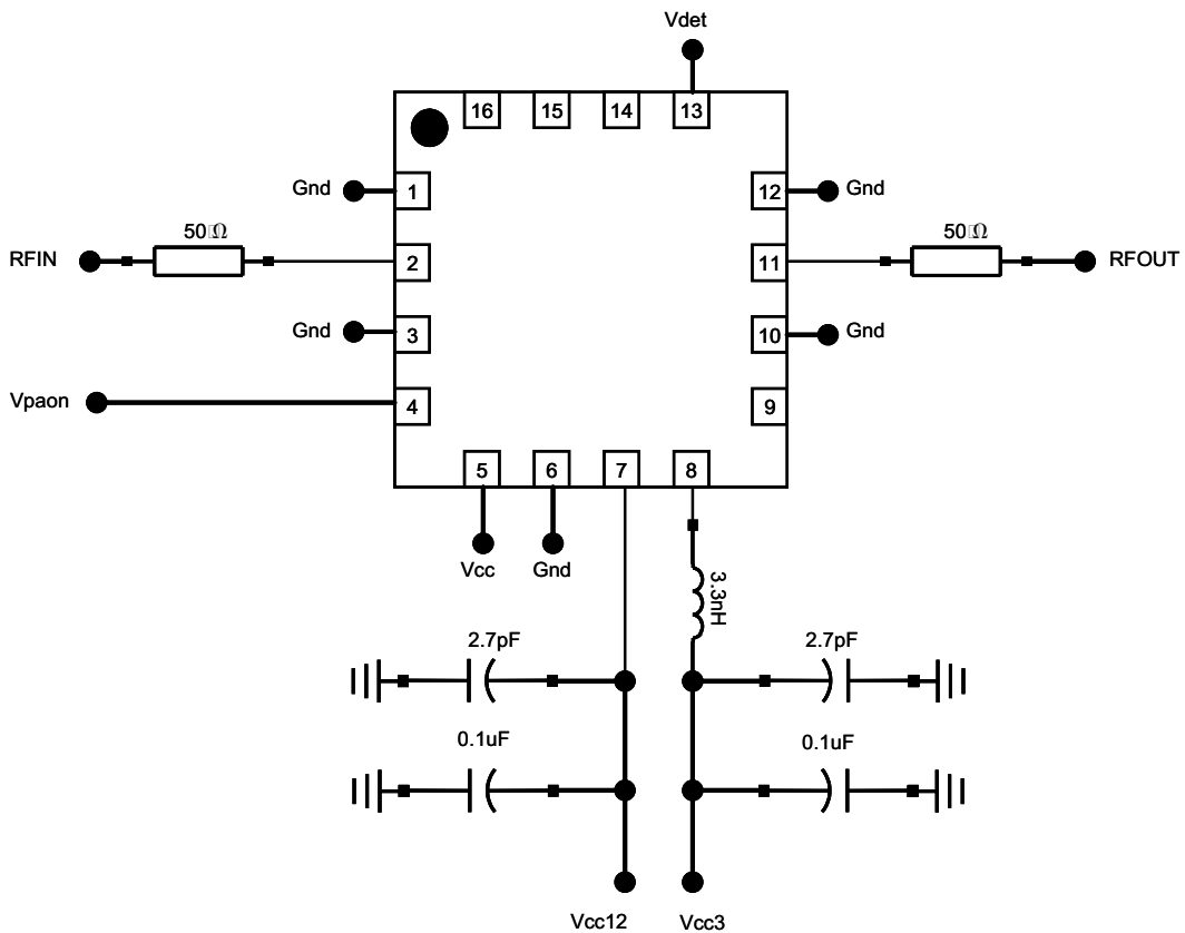
Figure 33: Application Circuit
