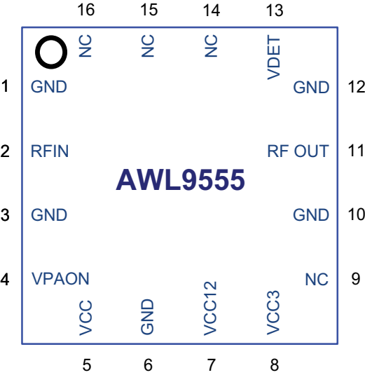
Figure 2: Pinout Diagram (Top View)
