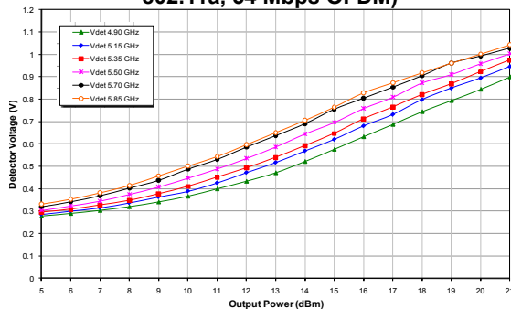
Figure 24: Voltage Detector vs. Output Power Across Frequency ( V_{cc} = +3.3 V, Temp = +25 °C 802.11a, 54 Mbps OFDM)
