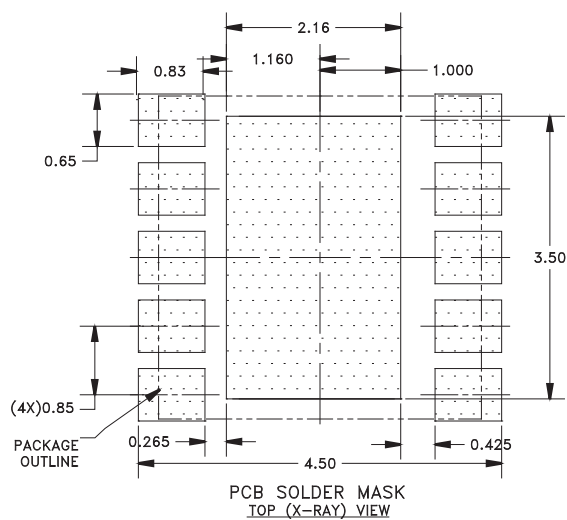
Figure 4: PCB Footprint
