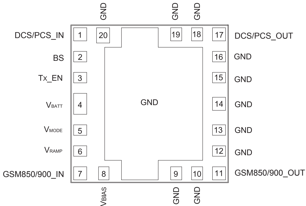
Figure 2: Pinout (X - ray Top View)
