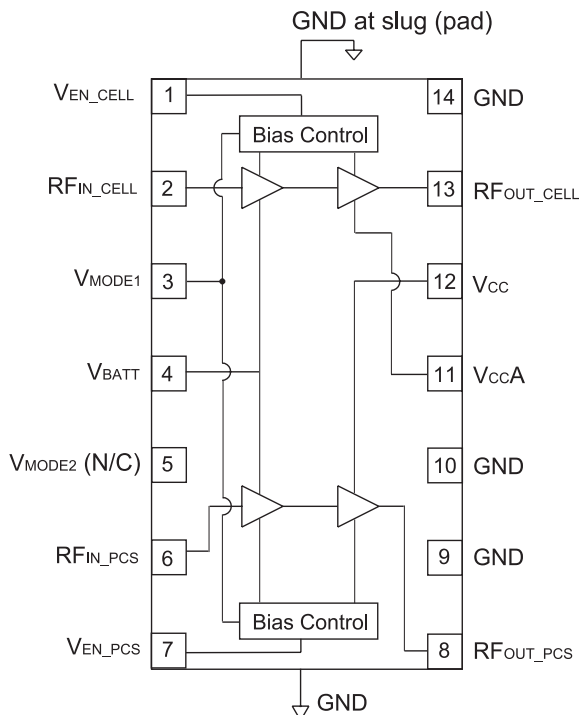
Figure 1: Block Diagram
