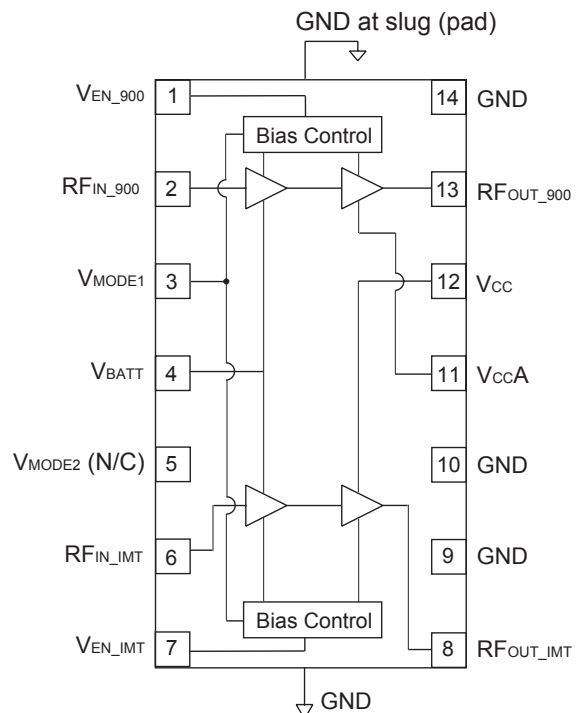
Figure 1: Block Diagram
