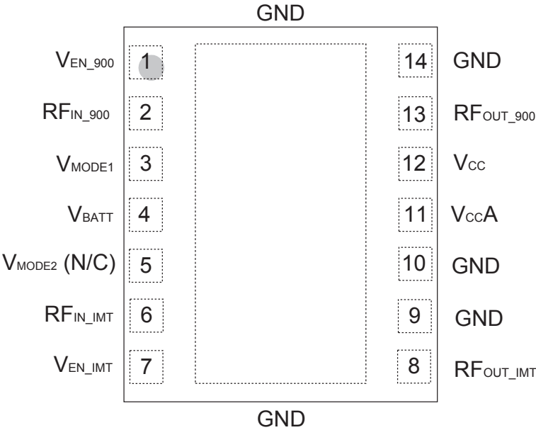
Figure 2: Pinout
