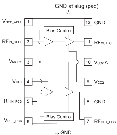
Figure 1: Block Diagram
