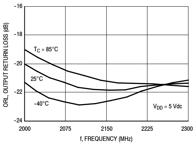
Figure 6. Output Return Loss ( S_{22} ) versus Frequency
