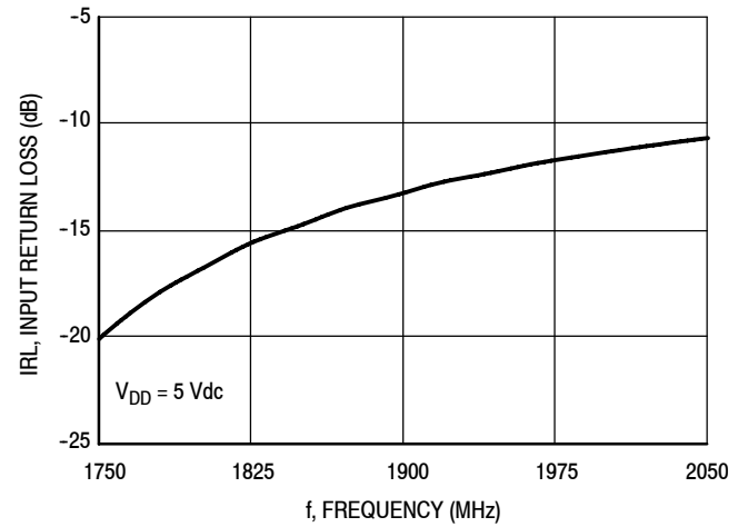
Figure 14. Input Return Loss (S11) versus Frequency
