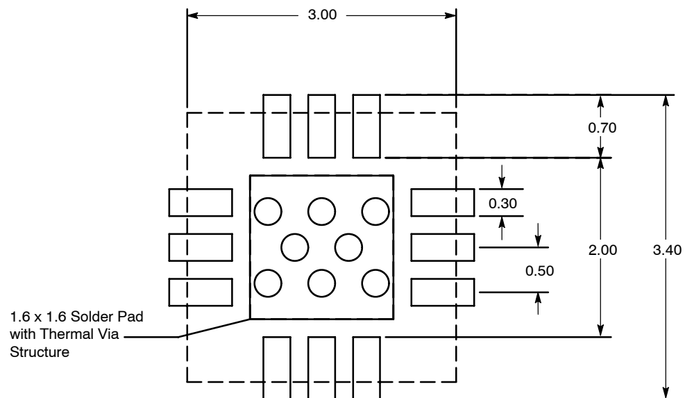
Figure 27. PCB Pad Layout for QFN 3x3
