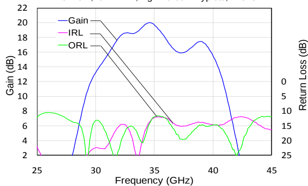
S-Parameters vs. Freq.
