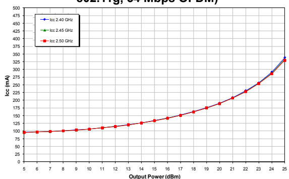
Figure 6: Tx Path I_{CC} vs. Output Power Across Frequency ( V_{CC} = +3.3 V, T_C = +25 °C, 802.11g, 54 Mbps OFDM)
