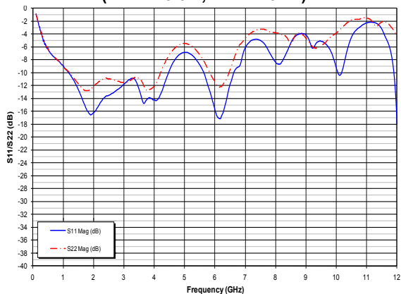
Figure 36: Bluetooth Path S11 & S22 Return Loss ( V_{CC} = +3.3\text{ V} , T_c = +25\text{ }^{\circ}\text{C} )
