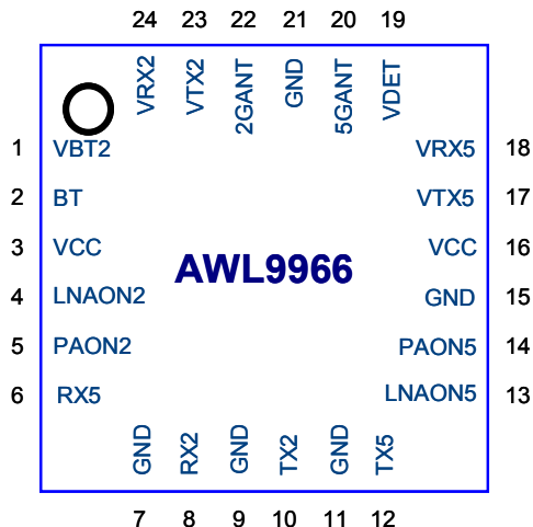
Figure 2: Pinout Diagram
