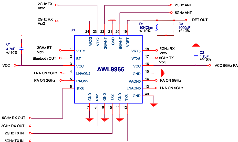
Figure 40: Application Circuit
