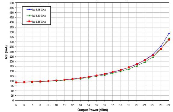
Figure 17: Tx Path ICC vs. Output Power Across Frequency ( T_c = +25\text{ }^\circ\text{C} , V_{CC} = +3.3\text{ V} , 802.11a, 54 Mbps OFDM)
