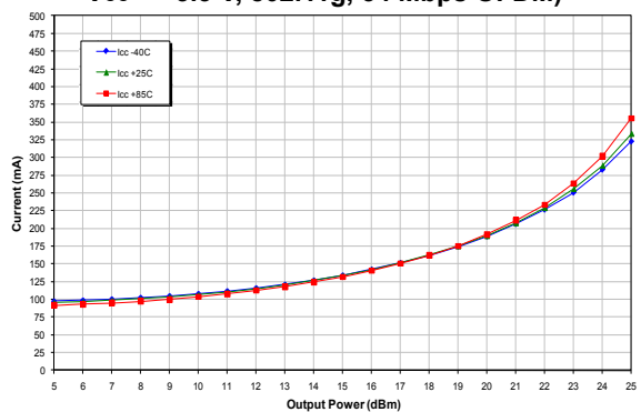
Figure 8: Tx Path I_{CC} vs. Output Power Across Temperature (Freq = 2.45 GHz, V_{CC} = +3.3 V, 802.11g, 54 Mbps OFDM)
