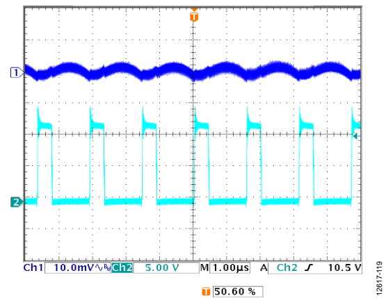
Figure 19. Steady State Waveform at Heavy Load, V_{IN} = 12\text{ V} , V_{OUT} = 3.3\text{ V} , I_{OUT} = 3\text{ A} , f_{SW} = 600\text{ kHz} , L = 4.7\text{ μH} , C_{OUT} = 47\text{ μF} \times 2 , FPWM Mode, Channel 1 = V_{OUTx} , Channel 2 = SWx
