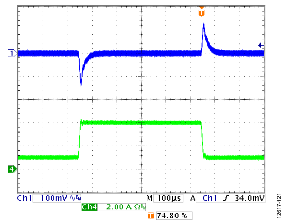
Figure 21. Channel 1/Channel 2 Load Transient, 1 A to 4 A, V_{IN} = 12\text{ V} , V_{OUT} = 3.3\text{ V} , f_{SW} = 600\text{ kHz} , L = 2.2\text{ μH} , C_{OUT} = 47\text{ μF} \times 2 , Channel 1 = V_{OUTx} , Channel 4 = I_{OUTx}
