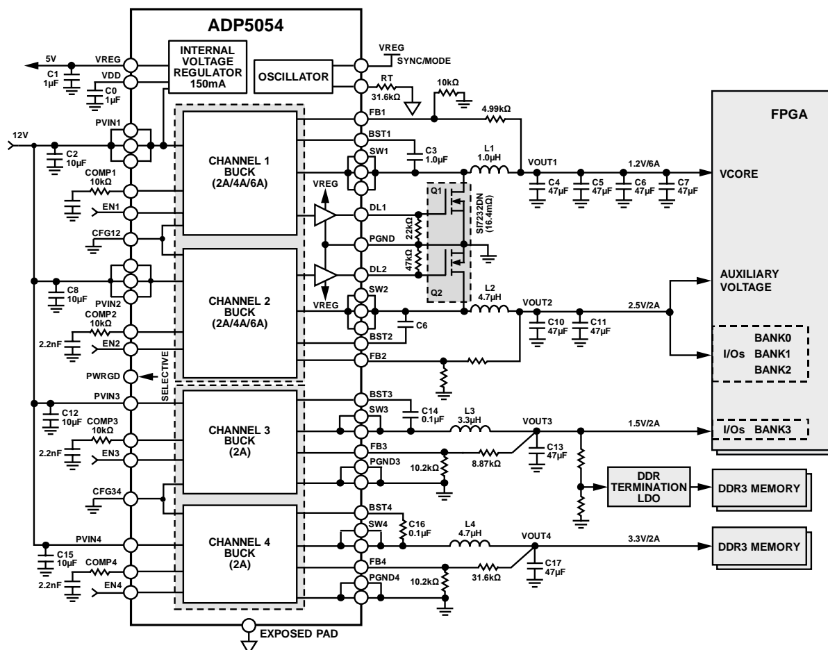
Figure 44. Typical Field Programmable Gate Array (FPGA) Application, 600 kHz Switching Frequency, Adjustable Output Model
