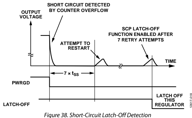
Figure 38. Short-Circuit Latch-Off Detection
