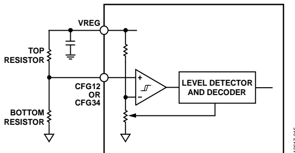
Figure 34. Level Detector Circuit for Soft Start
