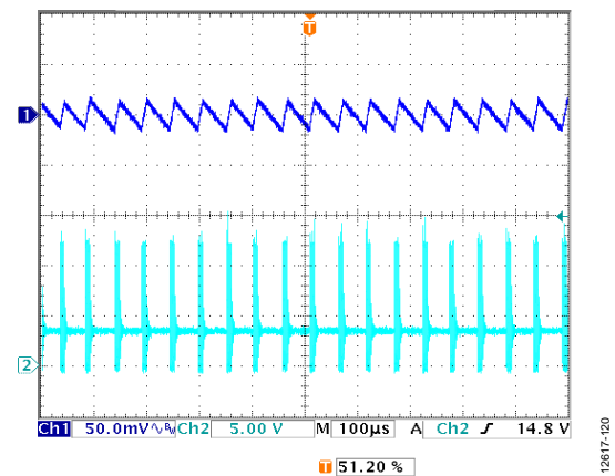
Figure 20. Steady State Waveform at Light Load, V_{IN} = 12\text{ V} , V_{OUT} = 3.3\text{ V} , I_{OUT} = 30\text{ mA} , f_{SW} = 600\text{ kHz} , L = 4.7\text{ μH} , C_{OUT} = 47\text{ μF} \times 2 , Automatic PWM/PSM Mode, Channel 1 = V_{OUTx} , Channel 2 = SWx
