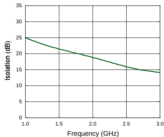
Isolation vs. Frequency, 25°C, 39 pF
