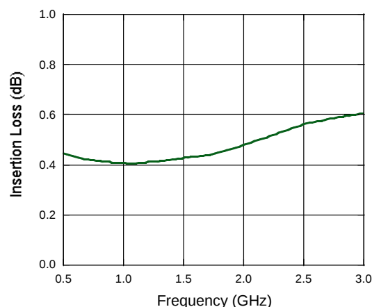
Insertion Loss vs. Frequency, 25°C, 39 pF
