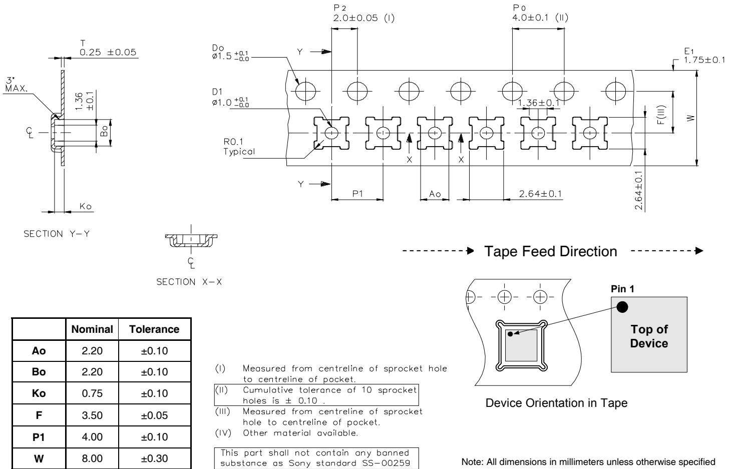
Figure 26. Tape and Reel Specifications
