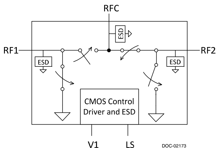
Figure 1. Functional Diagram
