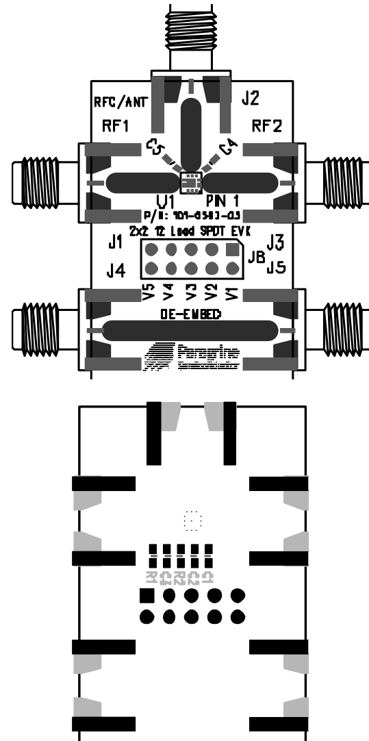
Figure 22. Evaluation Board Layout
