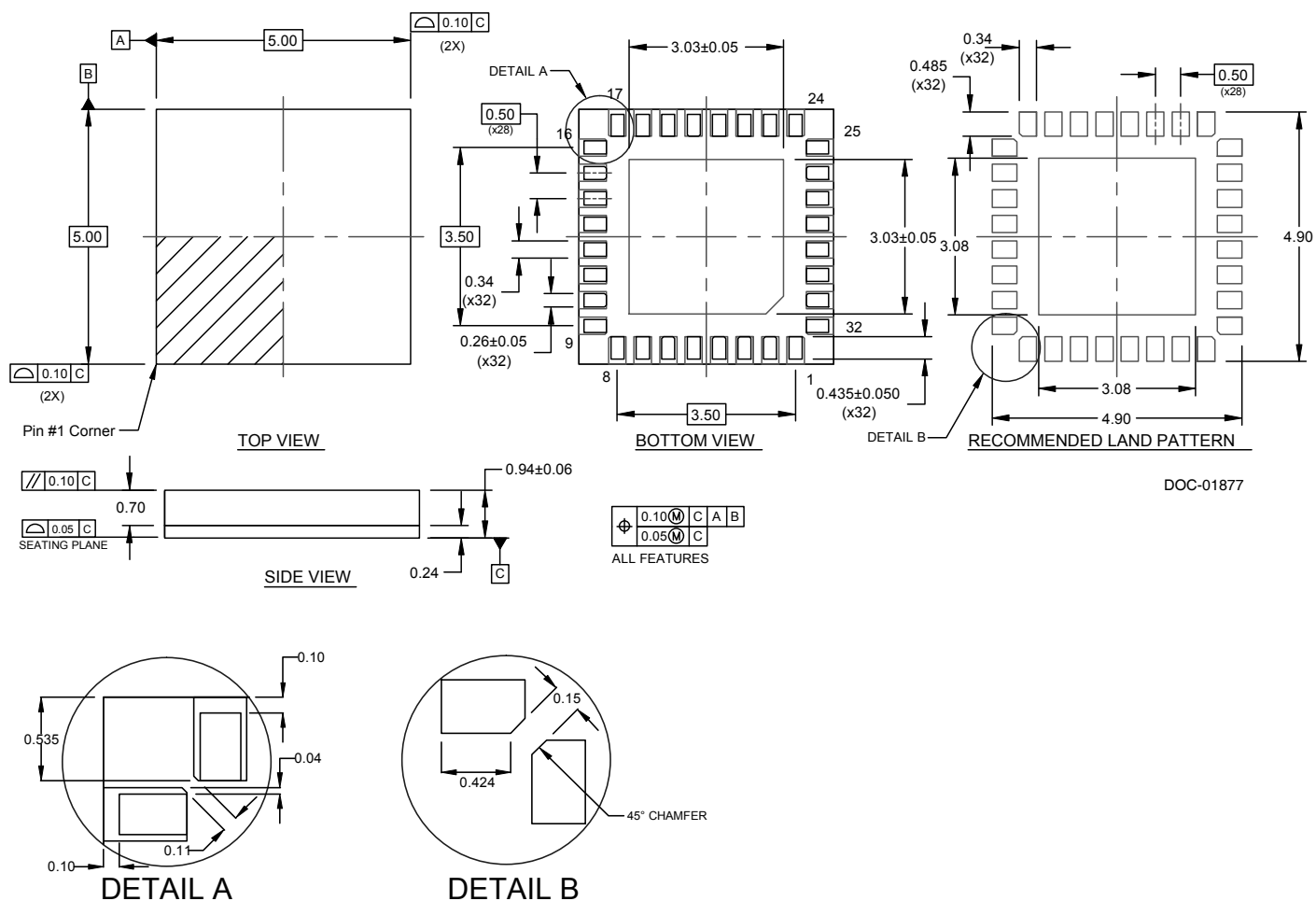
Figure 21. Package Drawing
