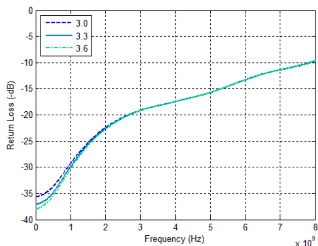
Figure 13. Terminated Port Return Loss vs. V_{DD}
