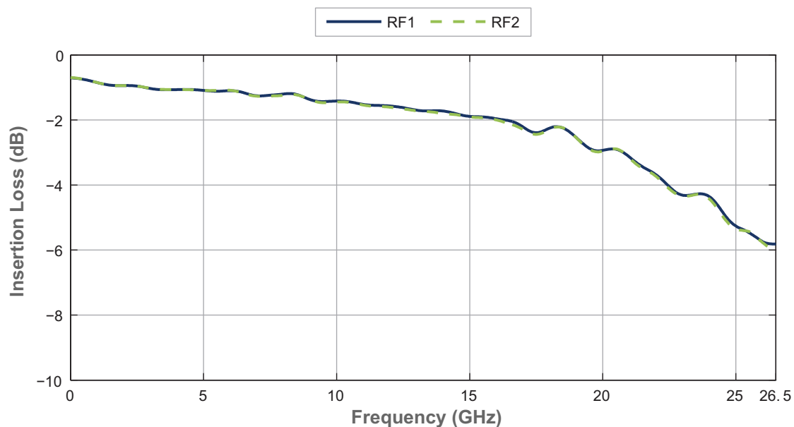
Figure 5 • Insertion Loss (RFC–RFX)(*)
