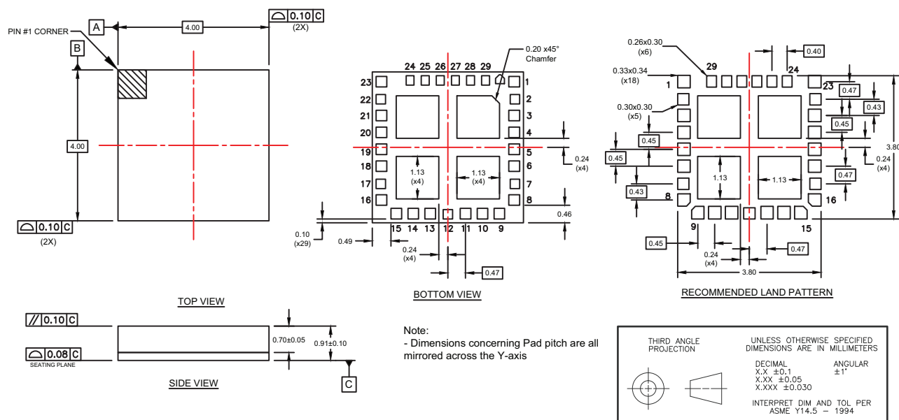
Figure 24 • Package Mechanical Drawing for 29-lead 4 × 4 × 0.91 mm LGA
