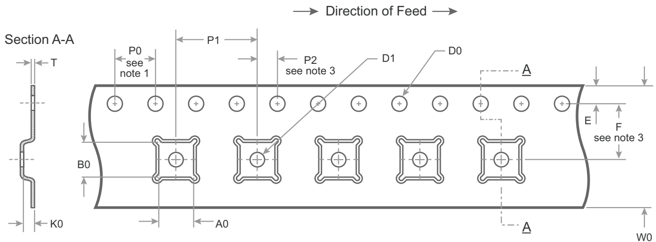
Figure 26 • Tape and Reel Specifications for 29-lead 4 \times 4 \times 0.91 mm LGA
