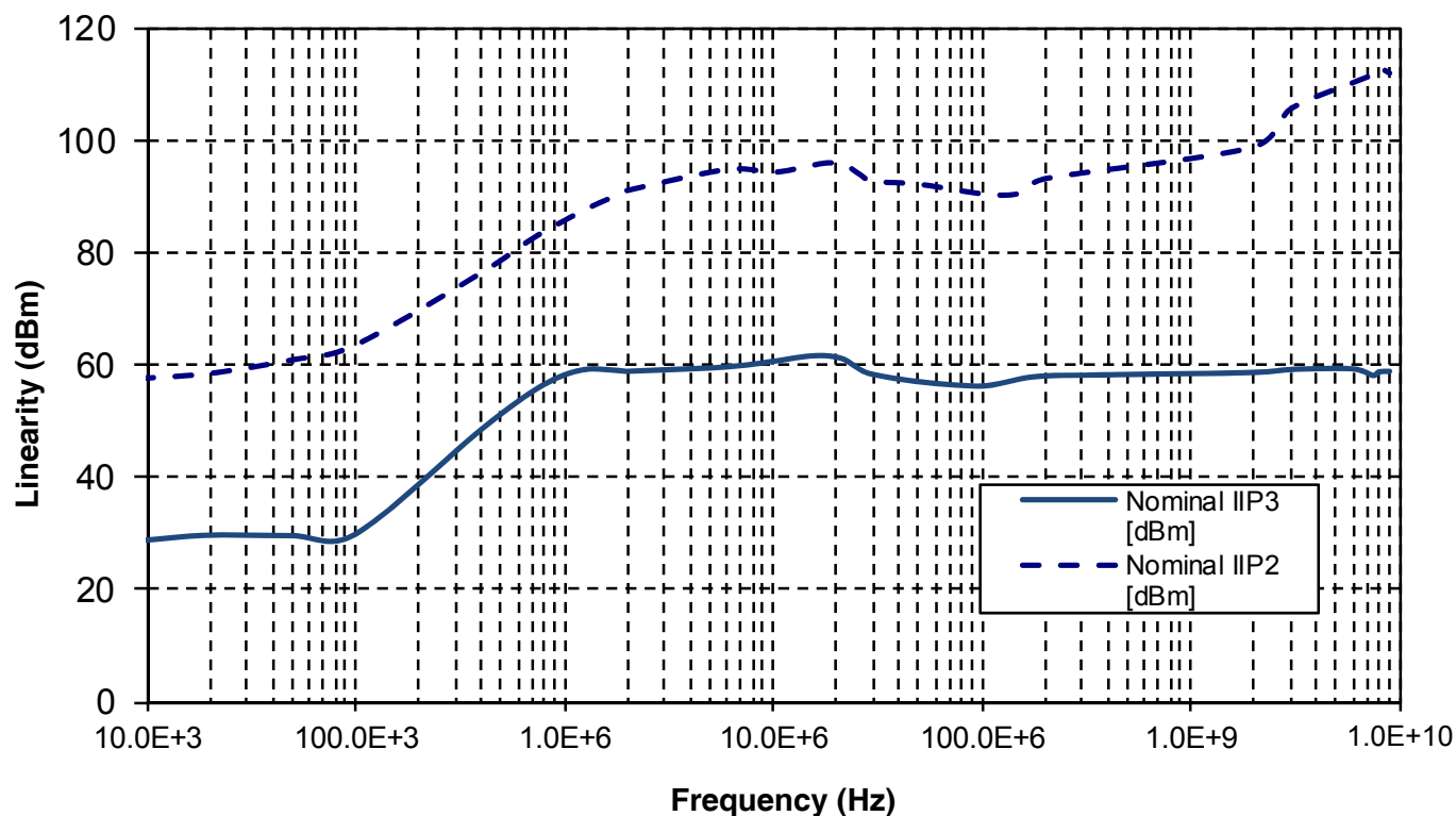
Figure 20. Linearity Performance (Temp = 25°C, V_{DD} = 3.3V , V_{SS} = 0 )
