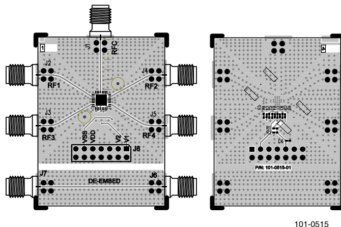
Figure 21. Evaluation Board Layouts
