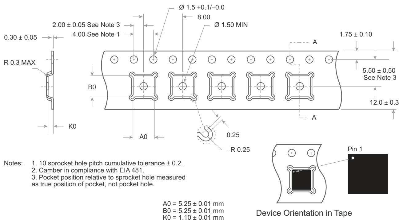
Figure 17 • Tape and Reel Specifications for 32-lead 5 × 5 mm QFN
