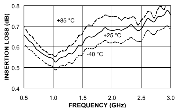
Insertion Loss Vs. Temperature
