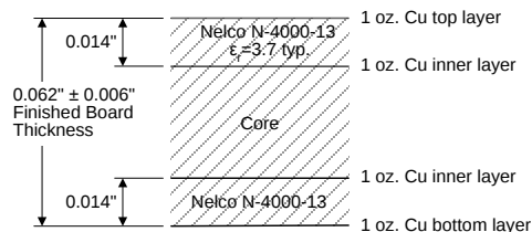
TriQuint PCB 1084809 Material and Stack-up
