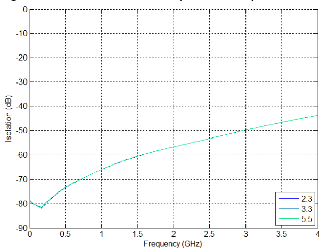
Figure 8. Isolation vs V_{DD} (RFC–RFX)
