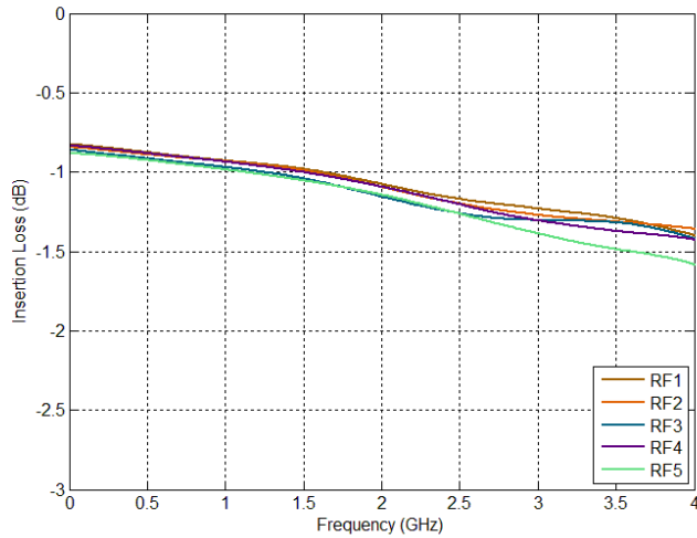
Figure 4. Insertion Loss (All Paths)
