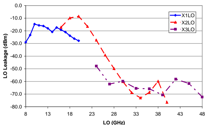
XU1005-QD, LO Leakage at RF (dBm), LO = +4 dBm
