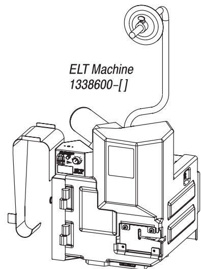
AMP-O-MATIC Side-Feed Stripper Crimper III Machine 1320895-[]
