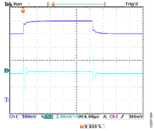
Figure 53. Line Transient Response, 2.5 V to 3 V, I_{LOAD} = 500\text{ mA} , Adjustable Version, V_{OUT} = 1.2\text{ V} , CH1 = V_{IN} , CH2 = V_{OUT}
