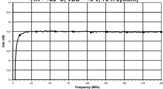
Figure 43: Low Frequency Applications (See Figure 20) Gain vs. Frequency - S24 Packaged (TA = +25° C; VDD = +8 V; 75 Ω system)
