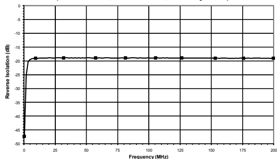
Figure 44: Low Frequency Applications (See Figure 20) Reverse Isolation vs. Frequency - S24 Packaged (TA = +25° C; VDD = +8 V; 75 Ω system)
