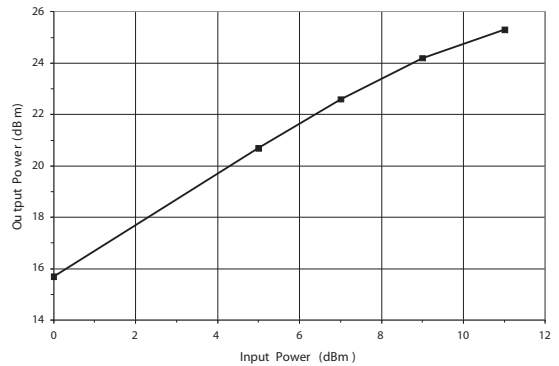
Figure 9: Output Power vs. Input Power - S3 Package Device ( T_A = +25\text{ }^\circ\text{C} ; V_{DD} = +8\text{ V} ; f = 500\text{ MHz} ; 75\ \Omega systems)
