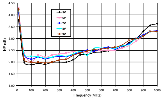
Figure 13: Noise Figure vs. Voltage S24 (SOT-89) Packaged Device (TA = +25 °C; 75 Ω systems)
