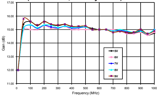
Figure 12: Gain vs. Frequency and Voltage S24 (SOT-89) Packaged Device (TA = +25 °C; 75 Ω systems)
