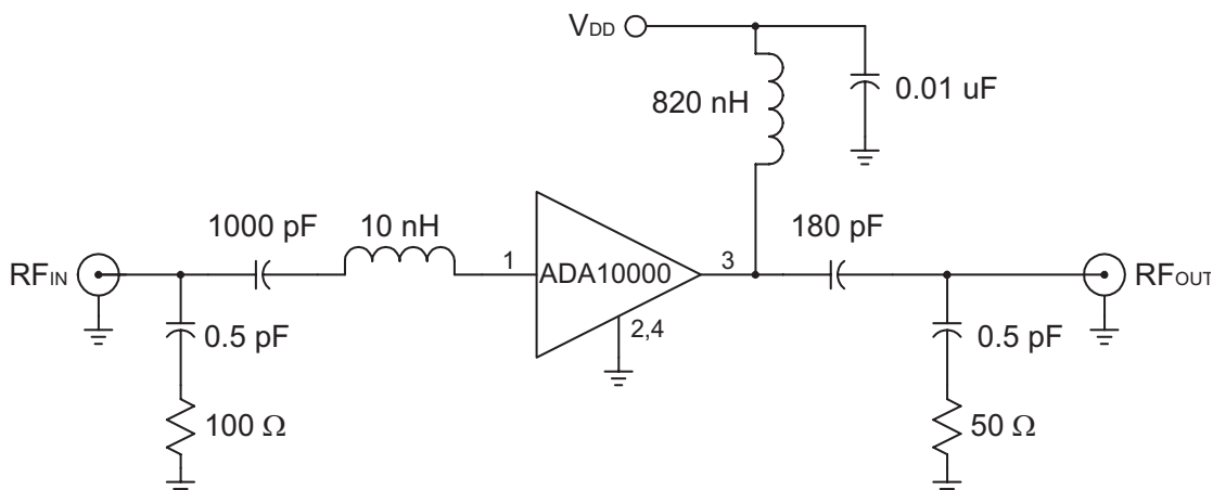
Figure 5: Standard Test/Application Circuit - S24 Packaged Device (75 Ω terminations)
