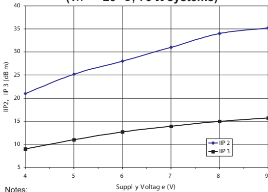
Figure 8: IIP2 and IIP3 vs. Supply Voltage - S3 Packaged Device ( T_A = +25\text{ }^\circ\text{C} ; 75\ \Omega systems)
