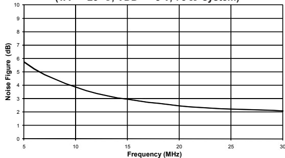
Figure 46: Low Frequency Applications (See Figure 20) Noise Figure vs. Frequency - S24 Packaged (TA = +25° C; VDD = +8 V; 75 Ω system)
