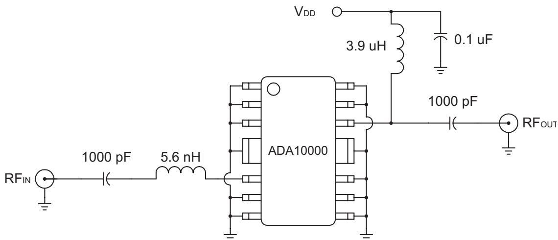
Figure 4: Standard Test/Application Circuit - S3 Packaged Device (75 Ω terminations)
