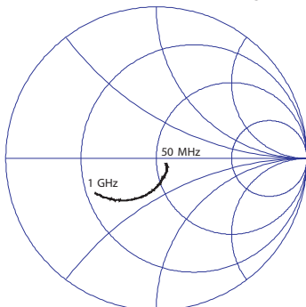
Figure 10: Unmatched Device Input Impedance S3 Packaged Device ( T_A = +25\text{ }^\circ\text{C} ; V_{DD} = +8\text{ V} ; 75\ \Omega systems)
