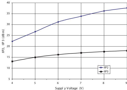
Figure 16: IIP2 and IIP3 vs. Supply Voltage - S24 Packaged Device (TA = +25 °C; 75 Ω systems)
