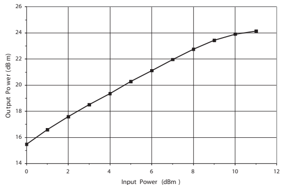
Figure 17: Output Power vs. Input Power - S24 Packaged Device (TA = +25 °C; VDD = +8 V; f = 500 MHz; 75 Ω systems)
