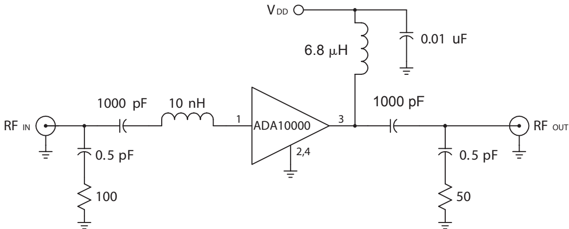
Figure 41: Low Frequency (5 MHz to 200 MHz) Test Application Circuit - S24 Packaged Device (75 Ω terminations)
