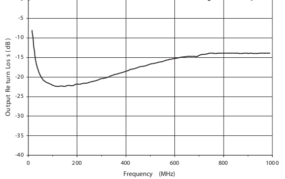
Figure 15: Output Return Loss vs. Frequency - S24 Packaged Device (TA = +25 °C; VDD = +8 V; 75 Ω systems)
