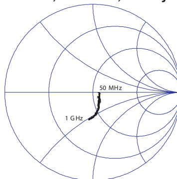
Figure 19: Unmatched Device Output Impedance - S24 Packaged Device ( T_A = +25\text{ }^\circ\text{C} ; V_{DD} = +8\text{ V} ; 75\ \Omega systems)
