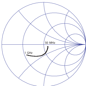
Figure 18: Unmatched Device Input Impedance - S24 Packaged Device ( T_A = +25\text{ }^\circ\text{C} ; V_{DD} = +8\text{ V} ; 75\ \Omega systems)
