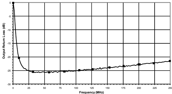
Figure 45: Low Frequency Applications (See Figure 20) Output Return Loss vs. Frequency - S24 Packaged (TA = +25° C; VDD = +8 V; 75 Ω system)
