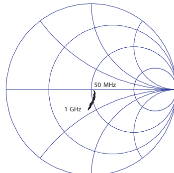
Figure 11: Unmatched Device Output Impedance - S3 Packaged Device ( T_A = +25\text{ }^\circ\text{C} ; V_{DD} = +8\text{ V} ; 75\ \Omega systems)
