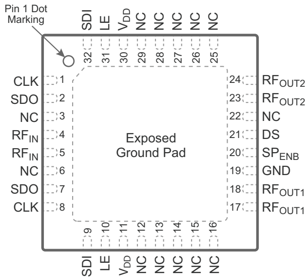
Figure 24 • Pin Configuration (Top View)
