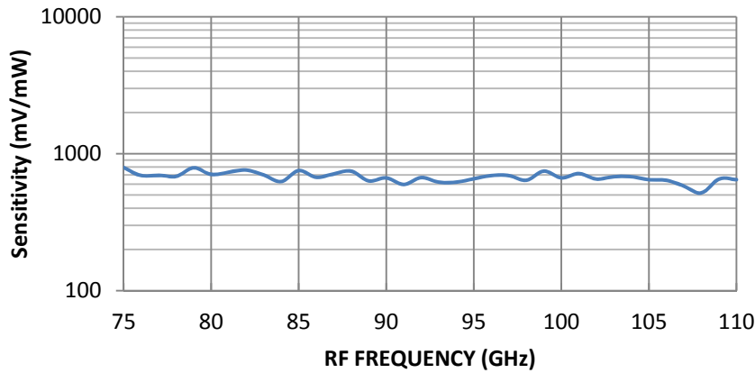
WR-10 Detector Sensitivity @ RF = -20 dBm
