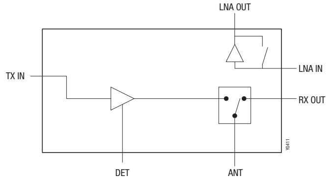
Figure 1. SKY85309-11 Block Diagram
