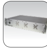
ZT-100 Network Analyzer Extender Ultra Reliable DC to 8.5 GHz 2 x 10 port switch matrix High Isolation, 90 dB typ Excellent VSWR, 1.2:1 typ
